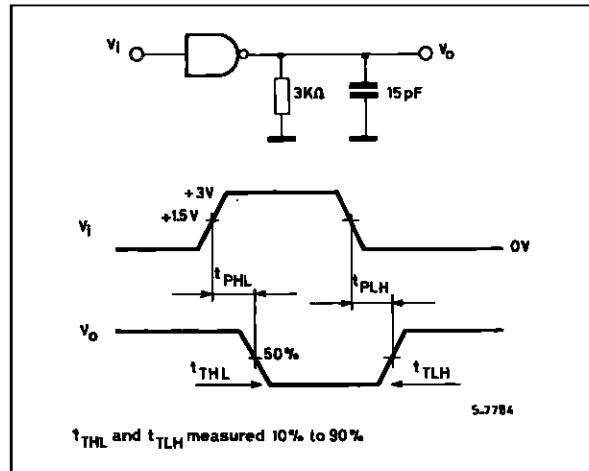
Figure 6 : Switching Response
